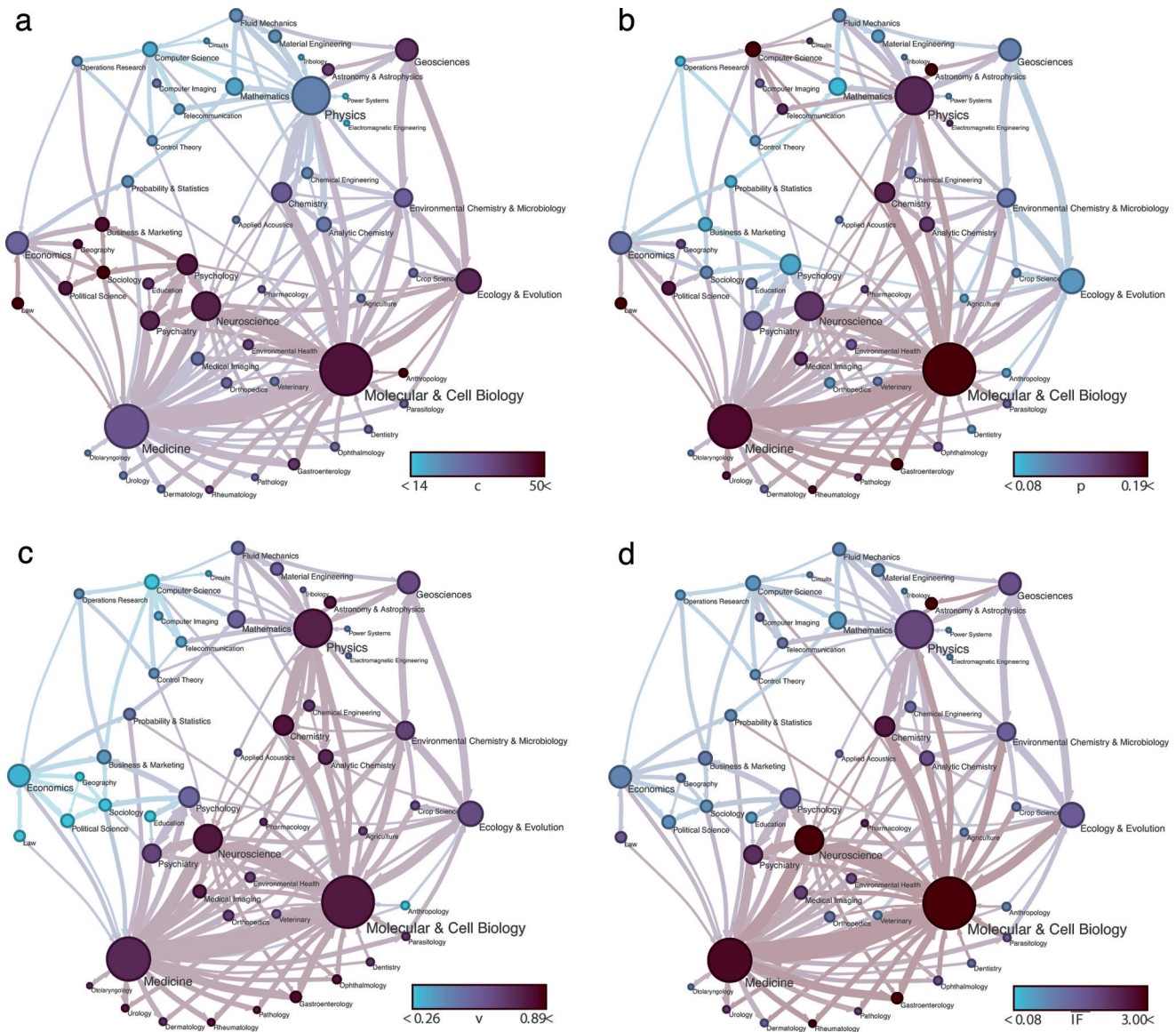
FIG. 2. Differences in citation patterns across fields. This figure illustrates the differences in c , p , v , and \overline{IF} across fields. Panel (a) shows differences in c , the average number of items cited per paper. Panel (b) shows differences in p , the fraction of citations to papers published in the two previous calendar years. Panel (c) shows differences in v , the fraction of citations to papers published in JCR-listed journals, and panel (d) shows differences in \overline{IF} , the weighted impact factor. Fields are categorized and mapped as in Rosvall and Bergstrom (2008).
